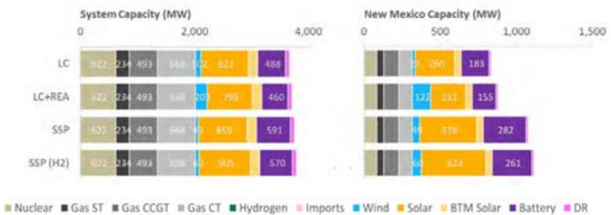
Figure 6-6. Capacity in 2031 by REA Case
