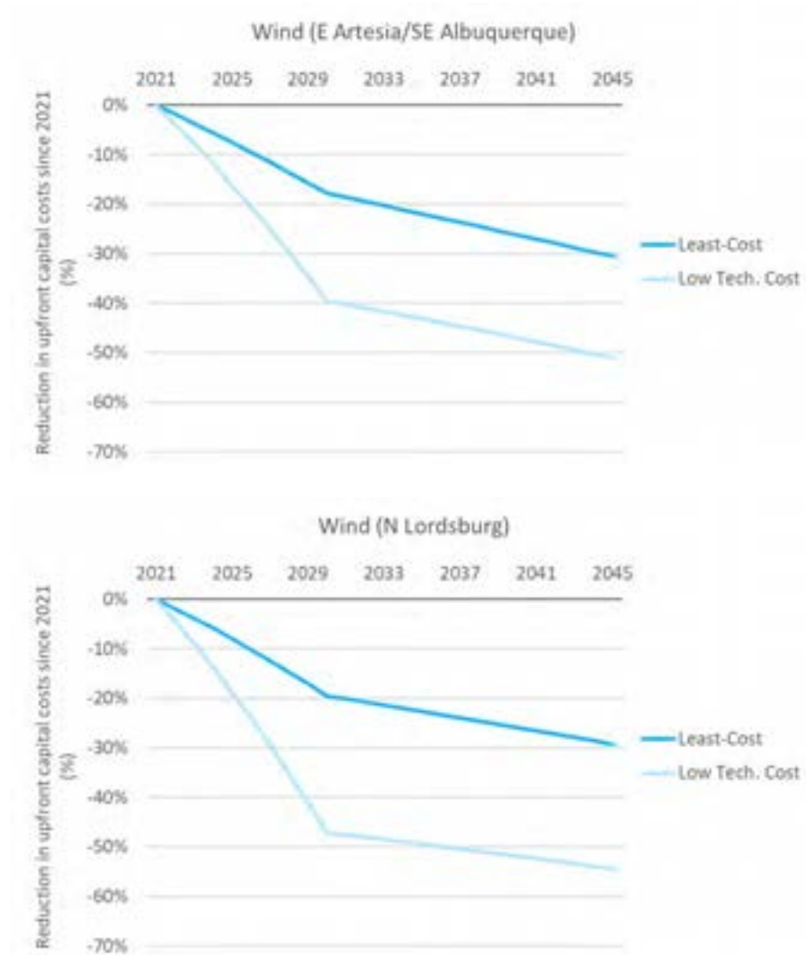
Figure 7-27. Cost Reductions in the Low Technology Cost Sensitivity
