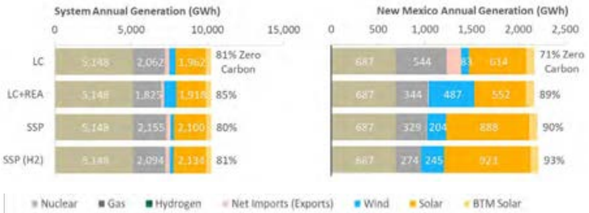
Figure 6-8. Annual Generation in 2031 by REA Case
