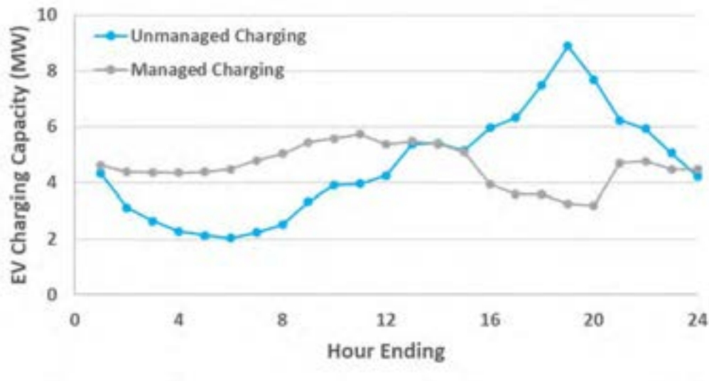
Figure 3-5. EV Charging Shape – Summer Weekday in 2030
