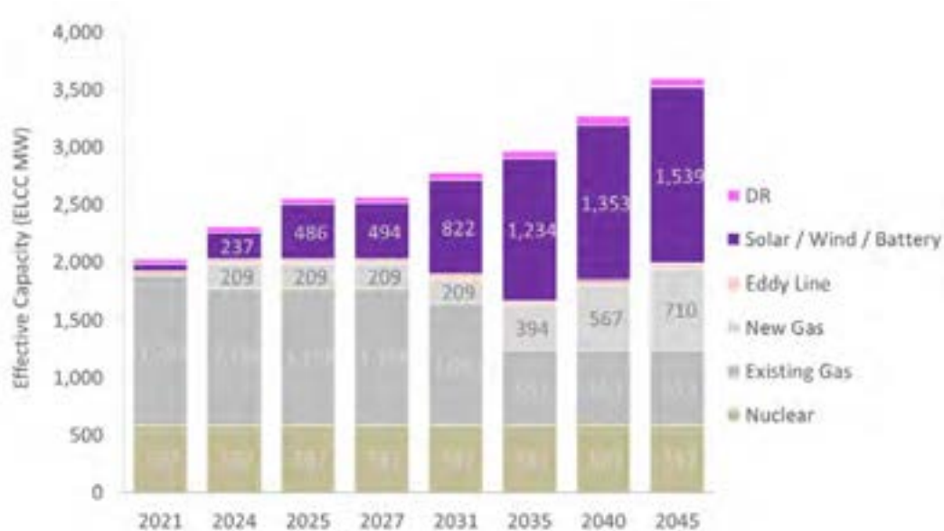
Figure 6-4. Effective Capacity in Least-Cost Case
