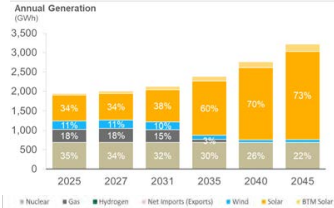
Figure 6-14. Annual Generation for NM Jurisdiction in SSP Case 41
