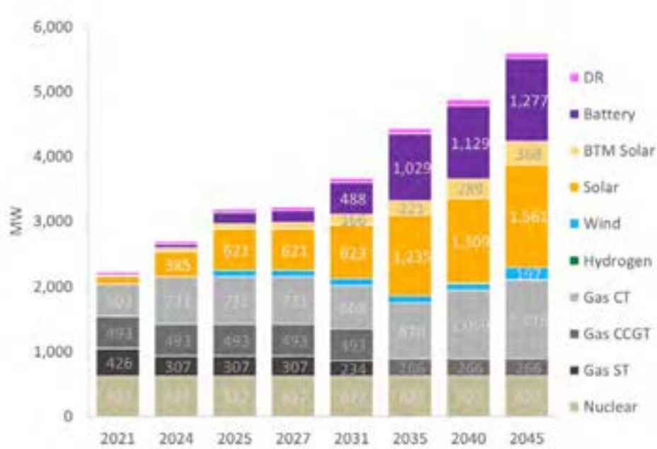
Figure 6-2. Total Capacity in Least-Cost Case
