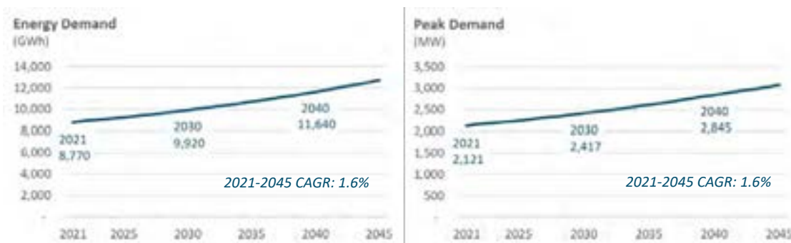
Figure 3-1. El Paso Electric Load Forecast 18
