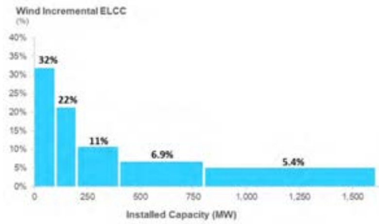
Figure 5-4. Wind Incremental ELCC
